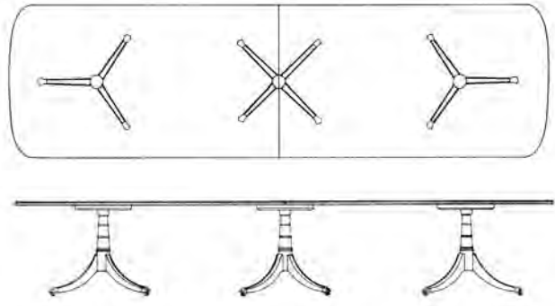
Rectangular top with "D" shaped ends, reeded edge, two KT-8501 (3-sweep) bases, and one KT-8601 (4-sweep) base.
