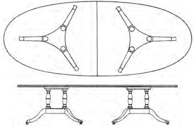
Oval top with reeded edge and two KT-8506 (3-sweep) bases.
