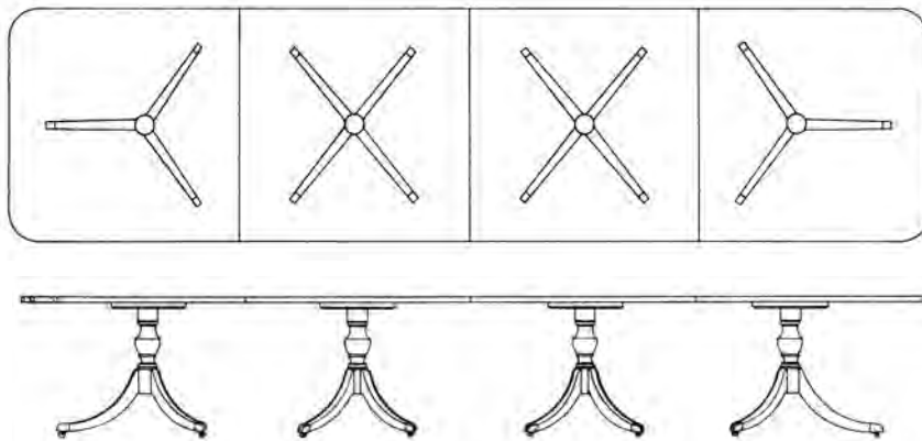
Rectangular top with rounded corners, square veneered edge, two KT-8503 (3-sweep) bases, and two KT-8603 (4-sweep) bases.
