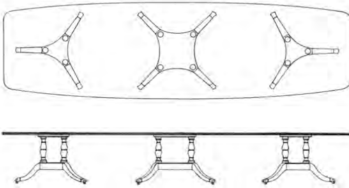
Boat shaped top with "D" shaped ends, bullnose edge, two KT-8506 (3-sweep) bases and one KT-8606 (4-sweep) base.
