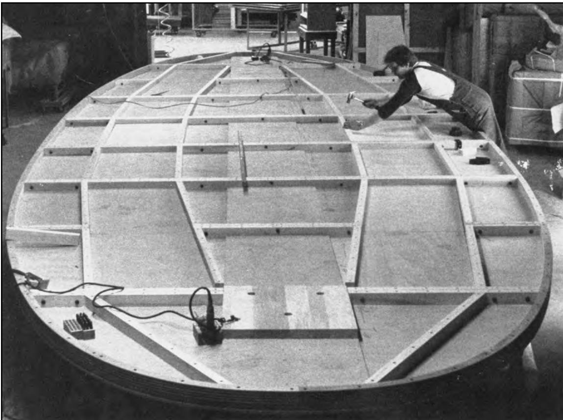
Maple cleating layout on underside of 9-section 36'x12' table for the summit conference at Williamsburg, Virginia. Craftsman shown stamping identification numbers to ensure proper set-up.
